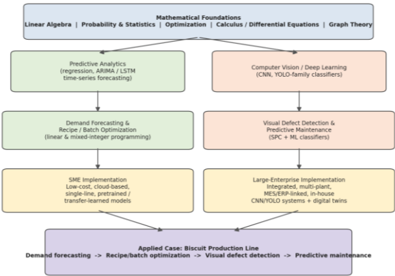
Figure1. Conceptual framework linking mathematical foundations
